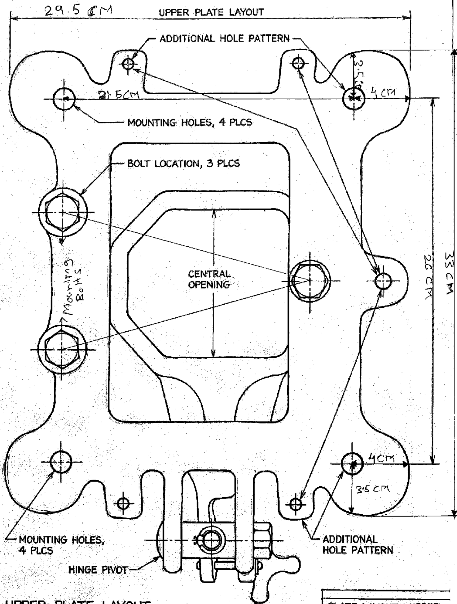
UPPER PLATE LAYOUT
